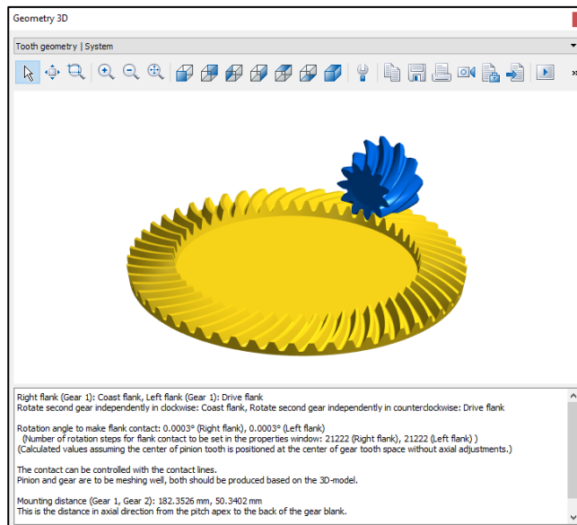
Figure 32. Display of the 3D bevel gear
