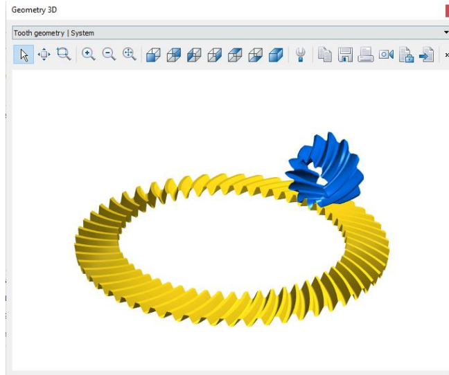
Figure 33. Bevel gears shown as skin models
