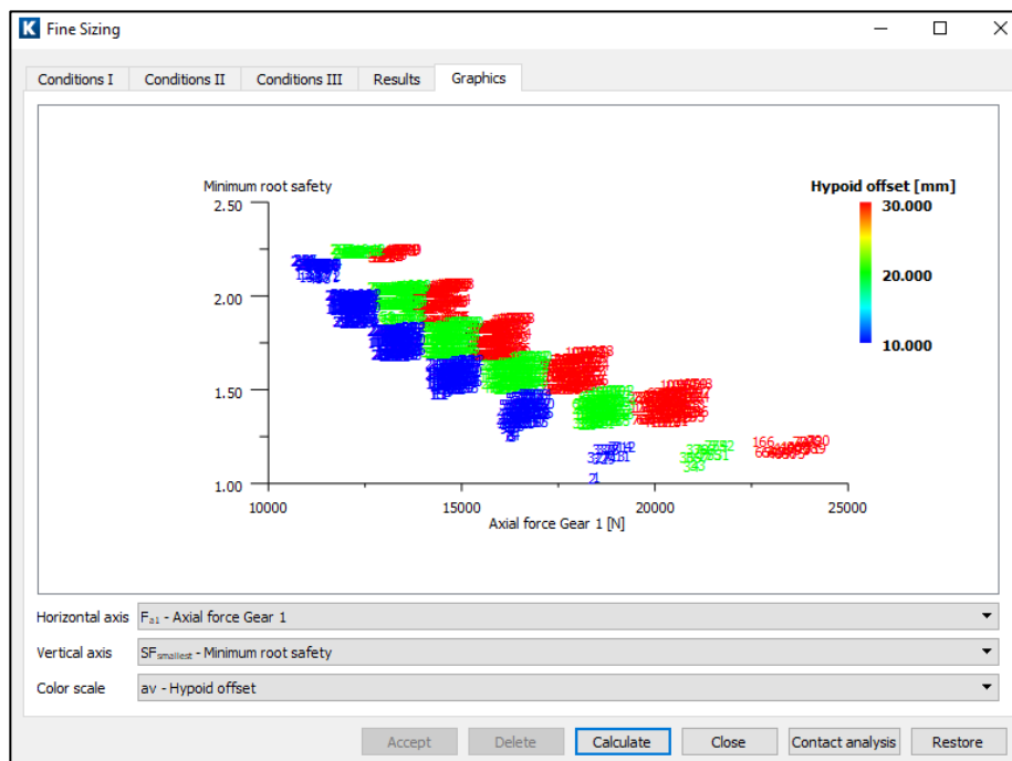
Figure 13. Displaying the results of fine sizing as a graphic
