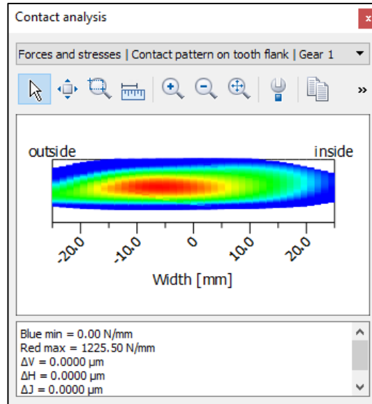
Figure 43. The graphic ‚contact lines on tooth flank‘ shows the contact pattern based on the contact lines.
