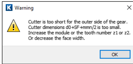
Figure 31. Warning if the palloid milling cutter is too small
