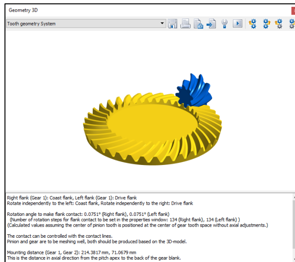
Figure 32. Display of the 3D bevel gear
