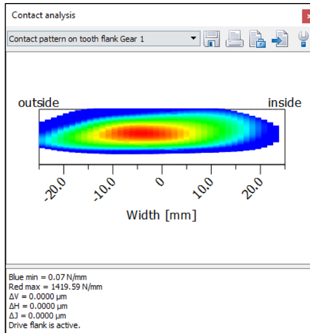
Figure 43. The graphic ‚contact lines on tooth flank‘ shows the contact pattern based on the contact lines.
