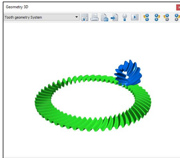
Figure 33. Bevel gears shown as skin models
