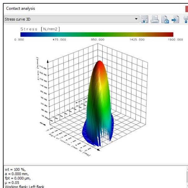
Figure 44. The graphic ‚stress curve 3D‘ allows the evaluation of stresses regarding stress peaks.
