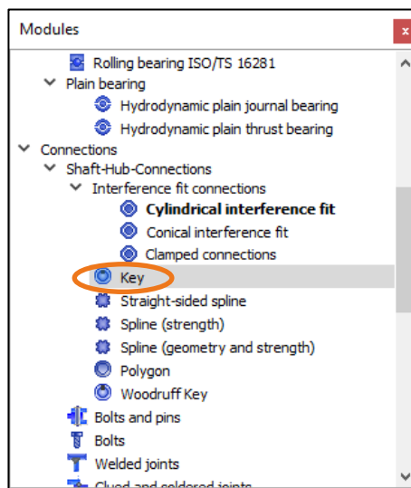
Figure 2. Selecting the «Key» calculation module under Shaft-Hub-Connections
