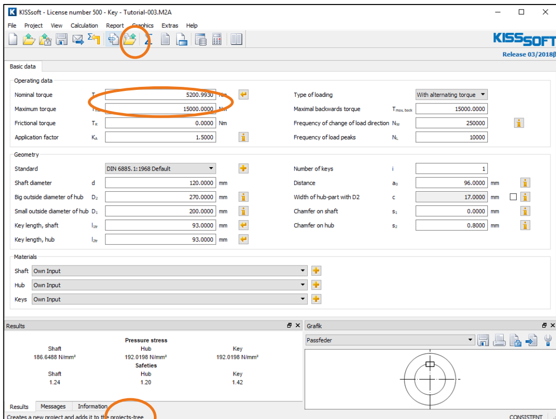
Figure 10. Defining the maximum permissible nominal torque
