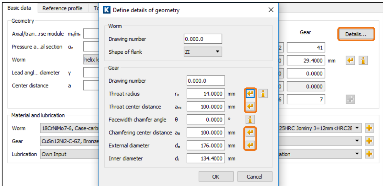
Figure 10. Calculating throat radius r_k , the external diameter d_e , throat center distance a_{rk} and chamfering center distance a_s
