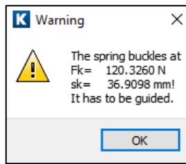
Figure 6. Warning shown if the spring will buckle and must be guided
