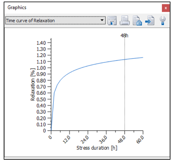
Figure 15. Relaxation time curve
