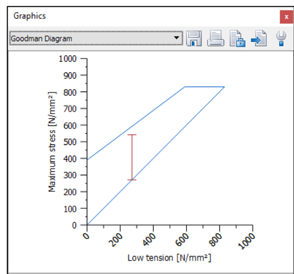
Figure 13. Goodman diagram
