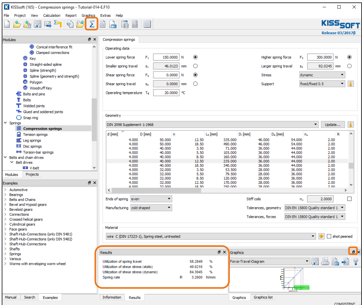
Figure 11. Calculating a compression spring
