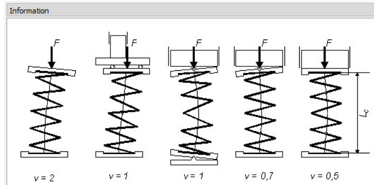
Figure 7. Support types with the corresponding support coefficients
