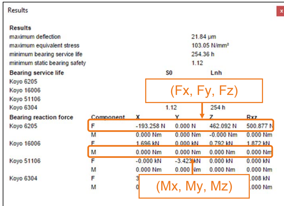
Figure 9. Components of bearing reaction forces and moments
