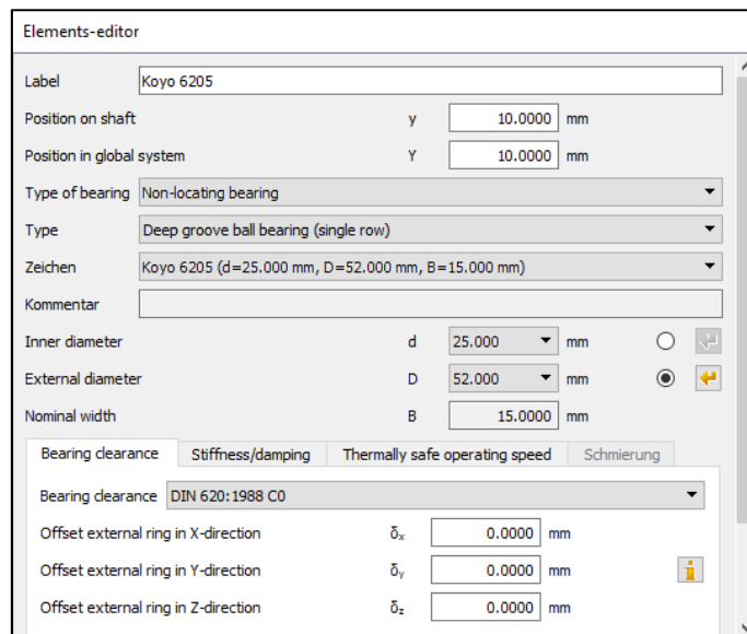
Figure 7. "Elements-editor" with roller bearing parameters
