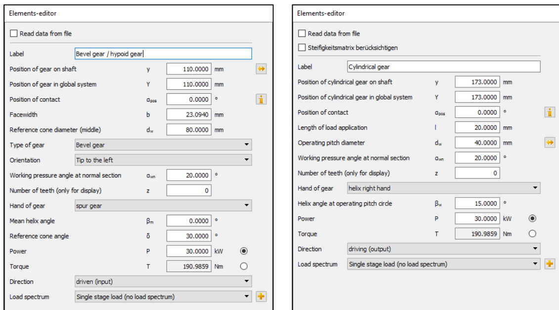
Figure 4. Definition of the force elements
