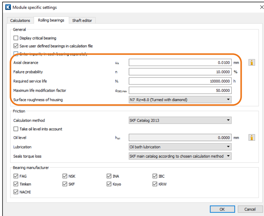
Figure 12. "Module specific settings" window in the "Roller bearing" tab with roller bearing parameters
