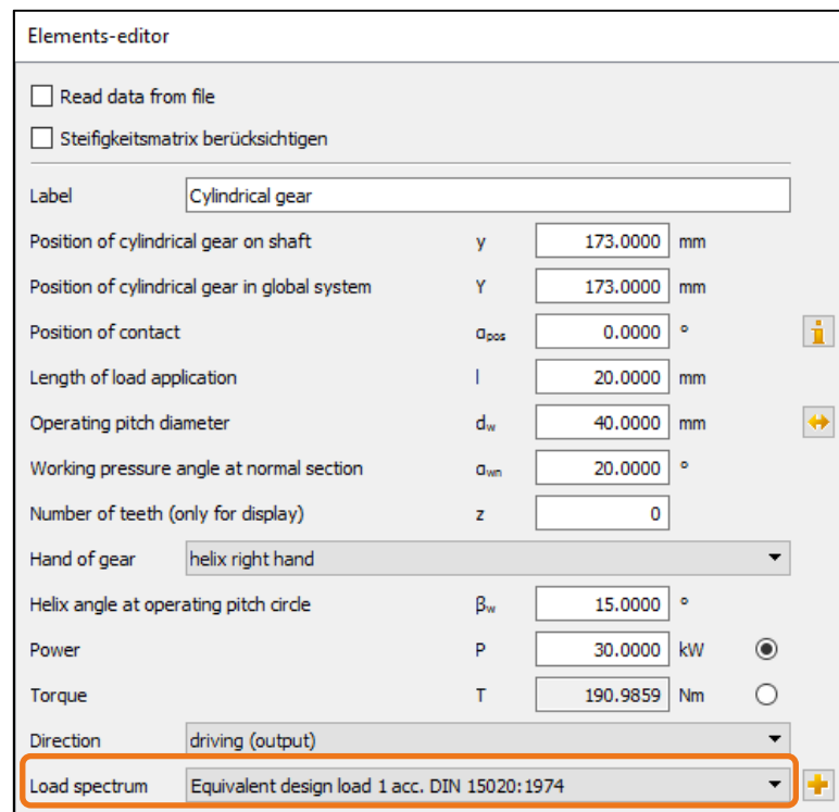
Figure 14. Example that takes a load spectrum into consideration for the force element cylindrical gear
