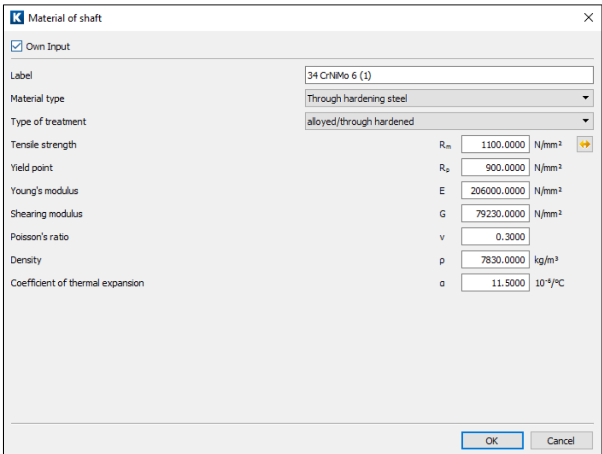
Figure 15. Defining a specific material
