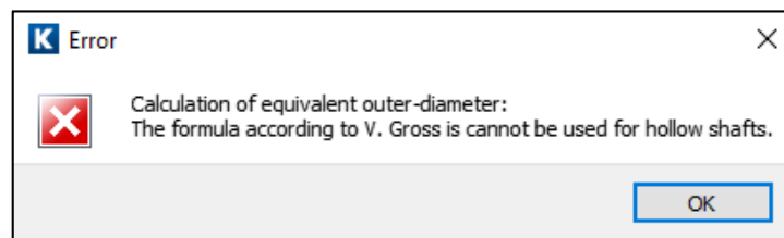
Figure 12. Error message
